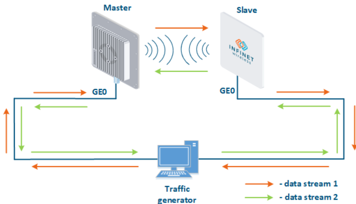
Figure - Bidirectional throughput test
