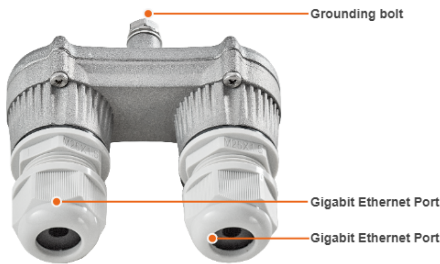
Figure - AUX-ODU-LPU-L
